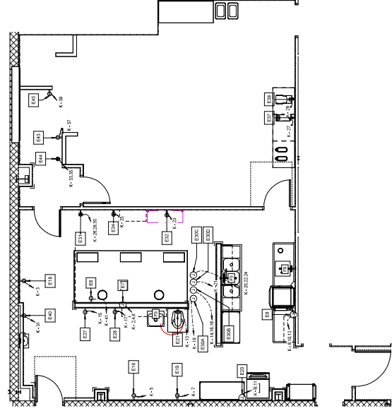
ENLARGED KITCHEN PLAN POWER
